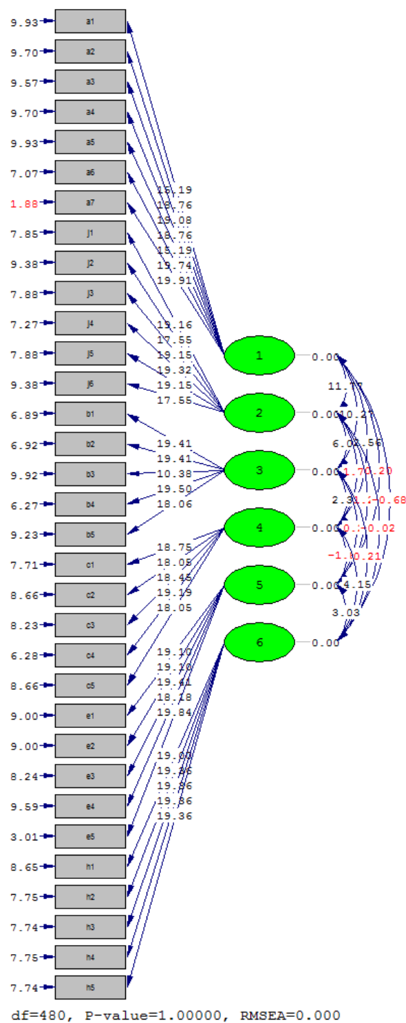
Fig.3 Factor analysis pattern in significant state Reference: (Researchers' findings)
