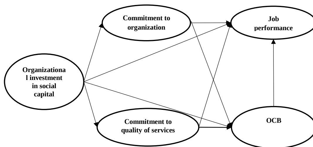
Fig1. Conceptual model
