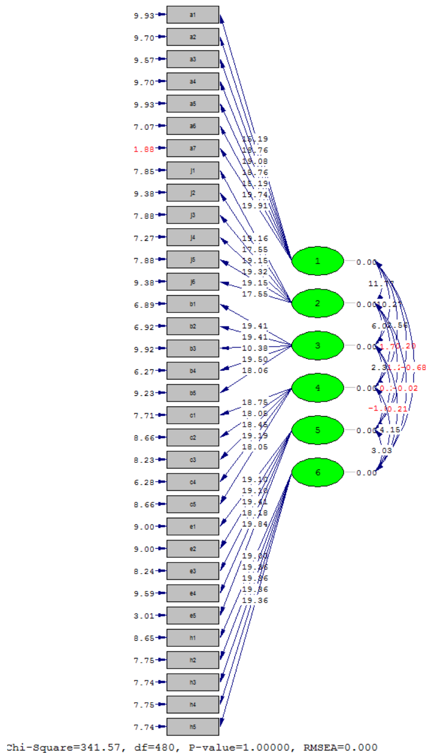
Fig.3 Factor analysis pattern in significant state
